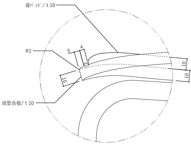
DETAIL A S=1/2
